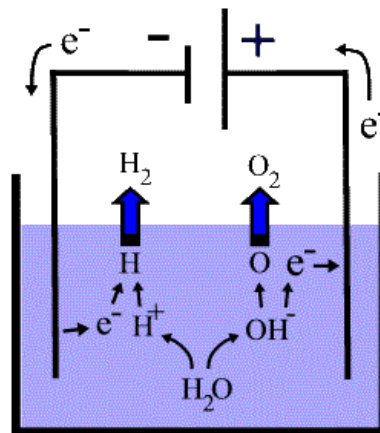
Figure 6: Electrolysis
