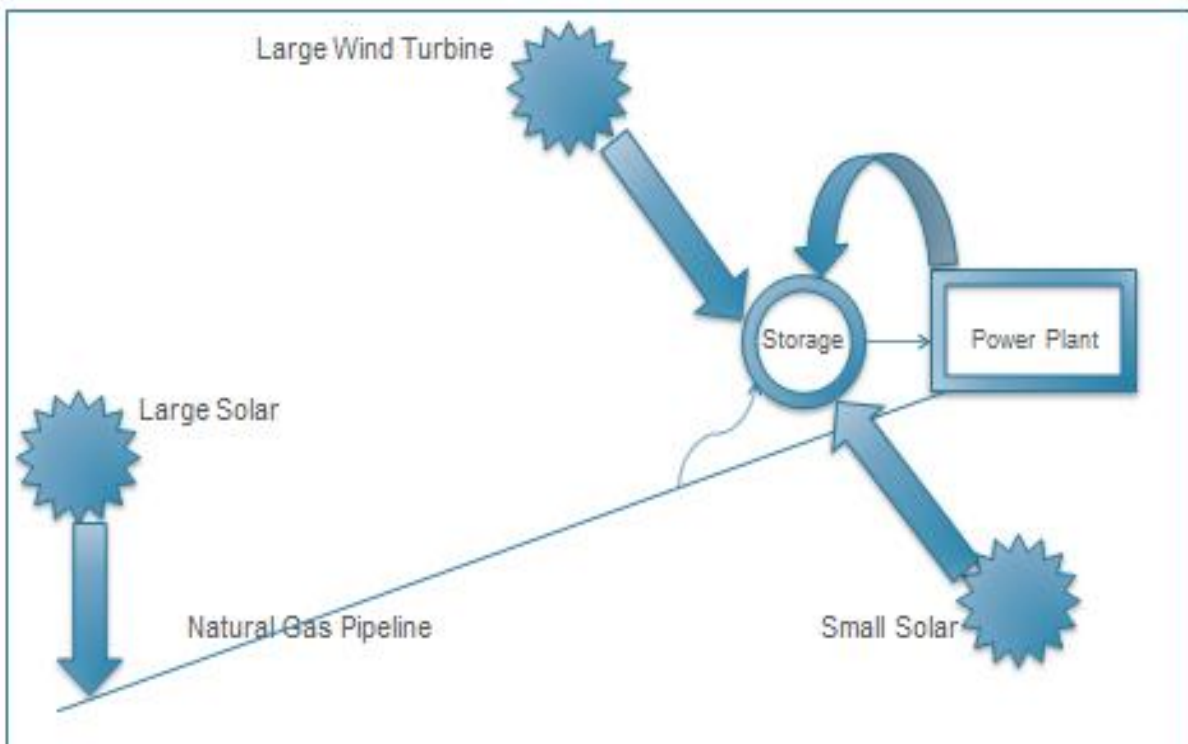
Figure 12: Flow Model
